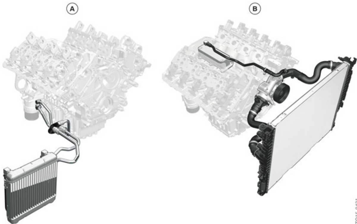
N62TU2 engine, installation of engine oil cooling components
